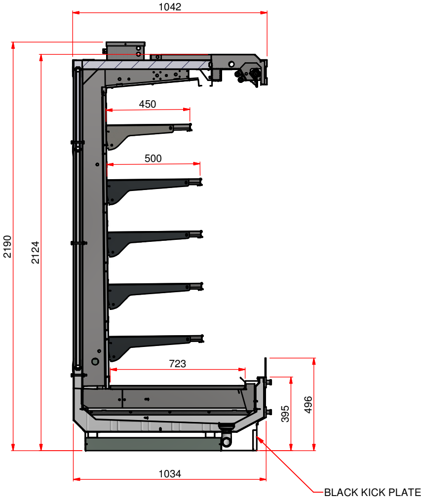
SIDE SECTION VIEW
