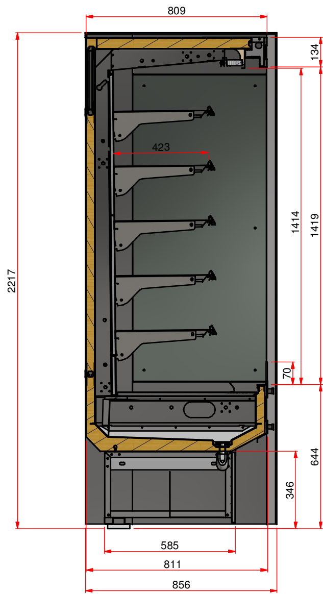
SIDE SECTION VIEW
