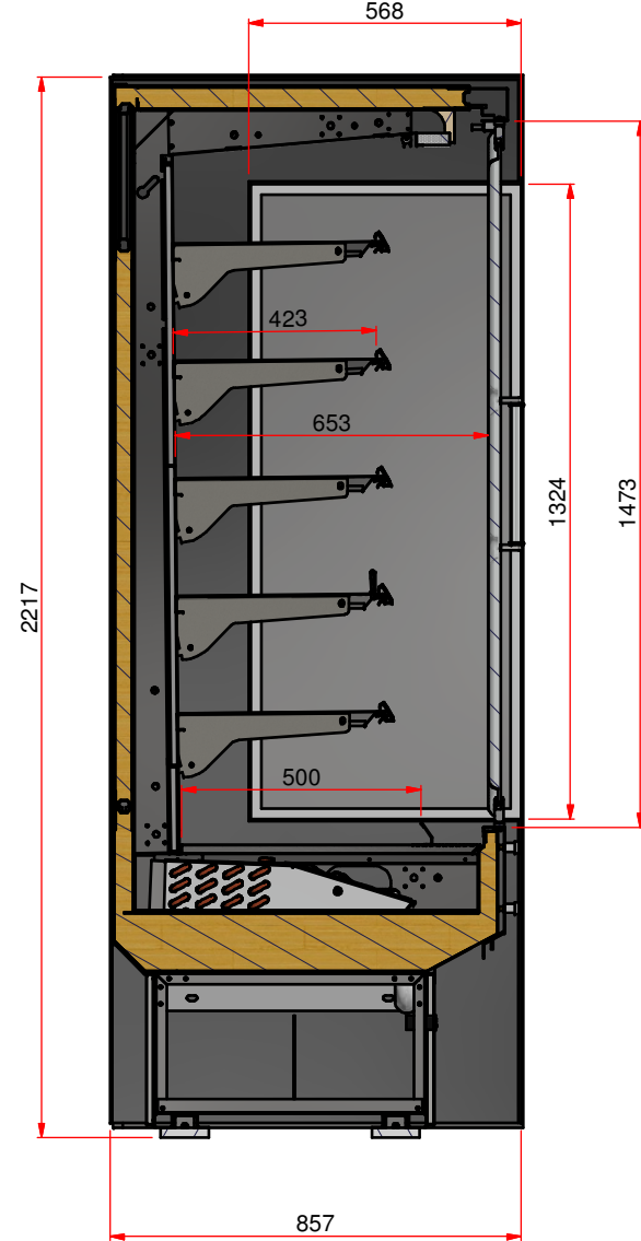
CLEAR VIEW DOORS SECTION VIEW
