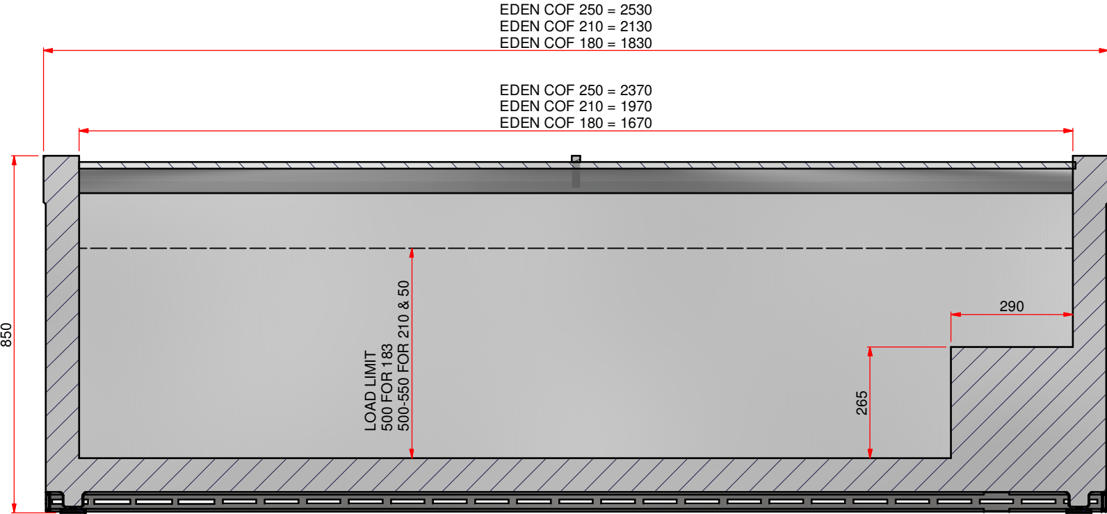
FRONT SECTION VIEW
