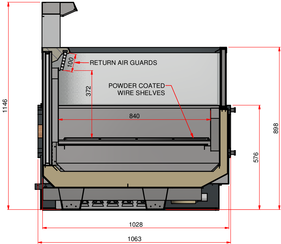
SIDE SECTION VIEW
