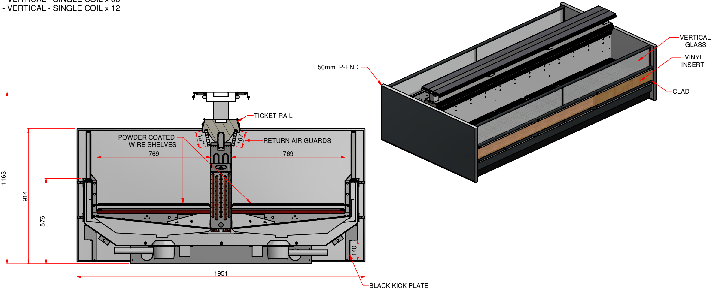
SIDE SECTION VIEW
