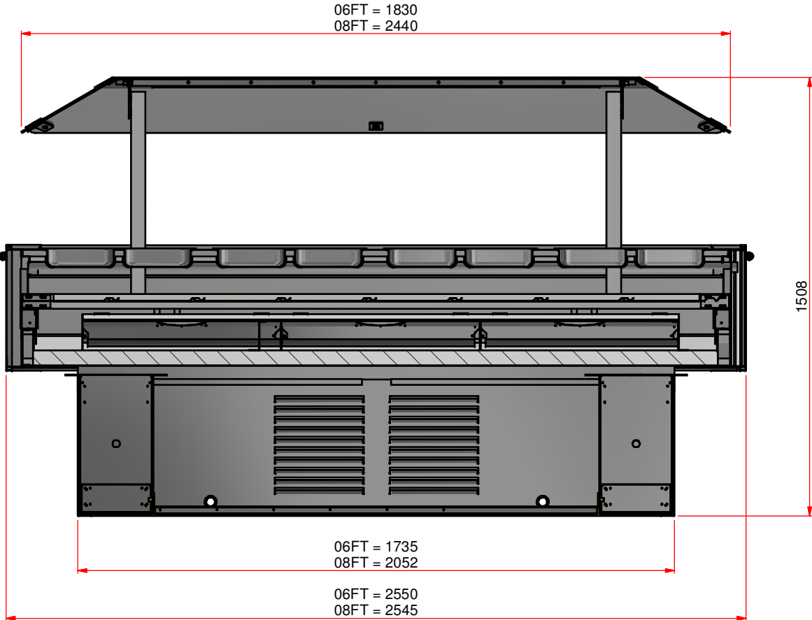
FRONT SECTION VIEW
