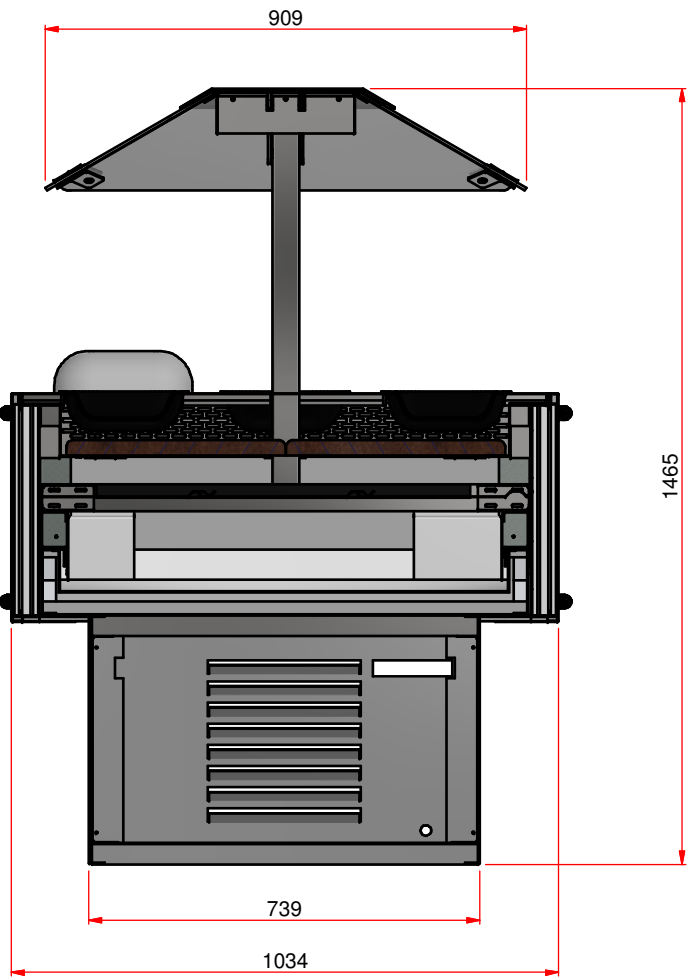
FRONT SECTION VIEW
