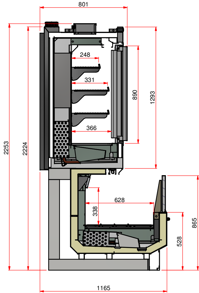
SIDE SECTION VIEW
