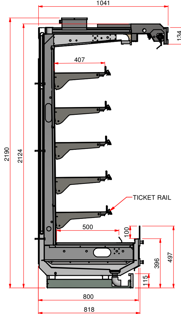
SIDE SECTION VIEW: EXTENDED CANOPY
