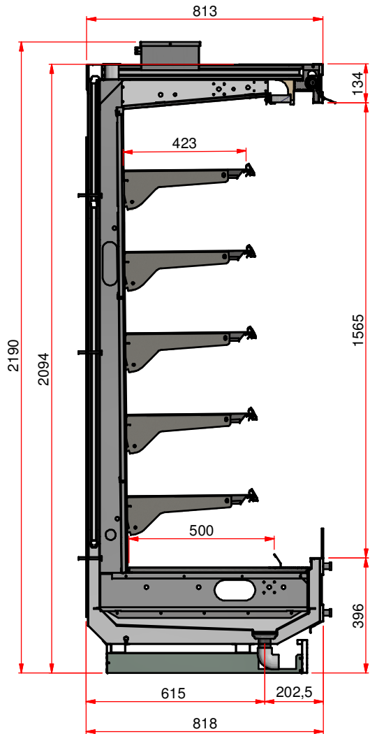
SIDE SECTION VIEW: INLINE CANOPY
