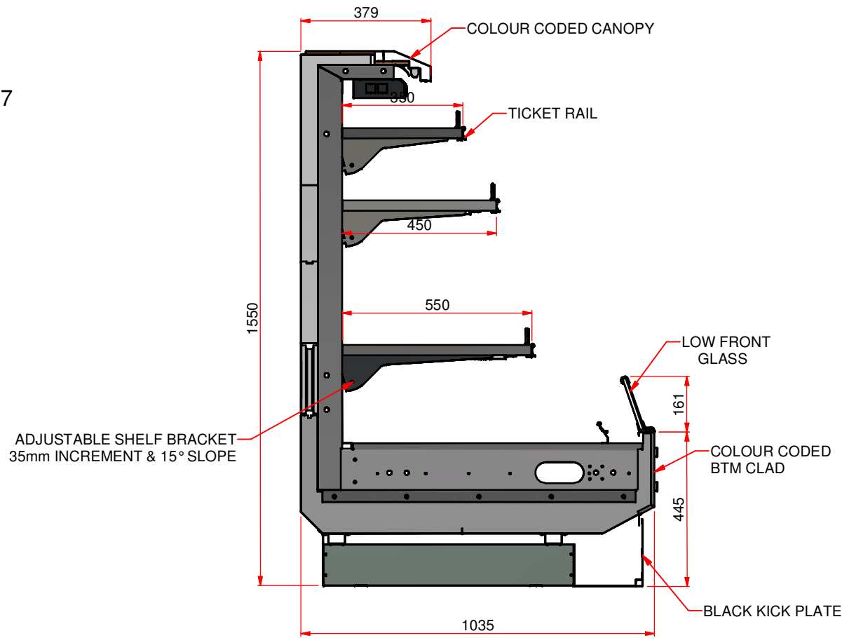
SIDE VIEW DIMENSIONS
