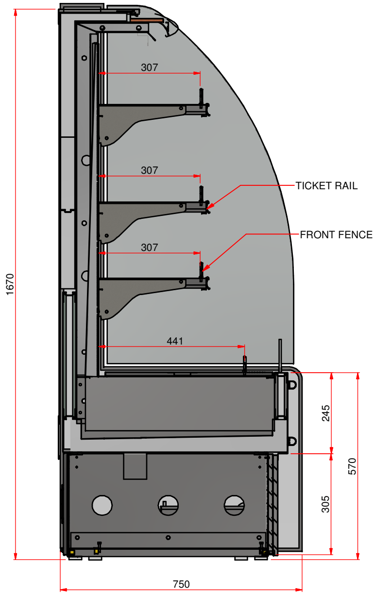
SIDE SECTION VIEW
