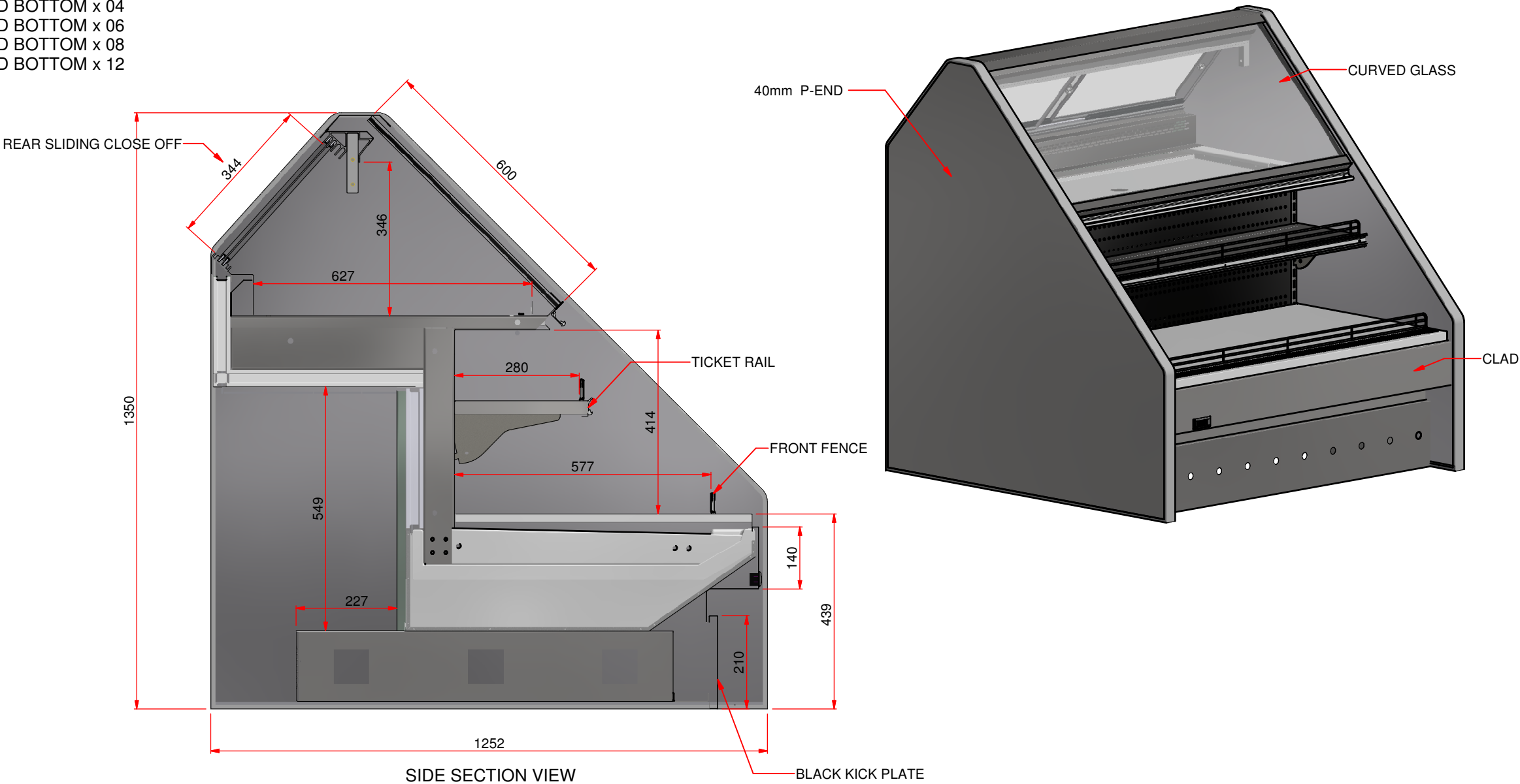
SIDE SECTION VIEW
